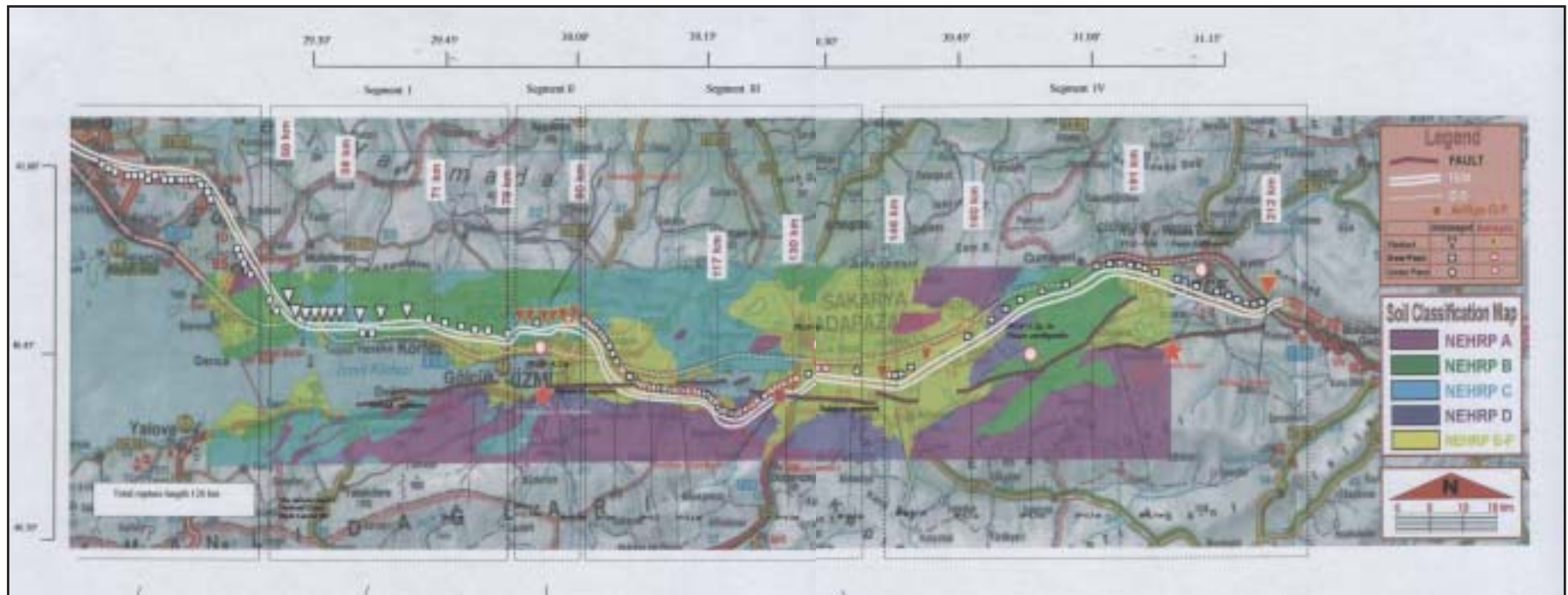
Figure 12 Damage distribution overlaid on a soil classification map.
