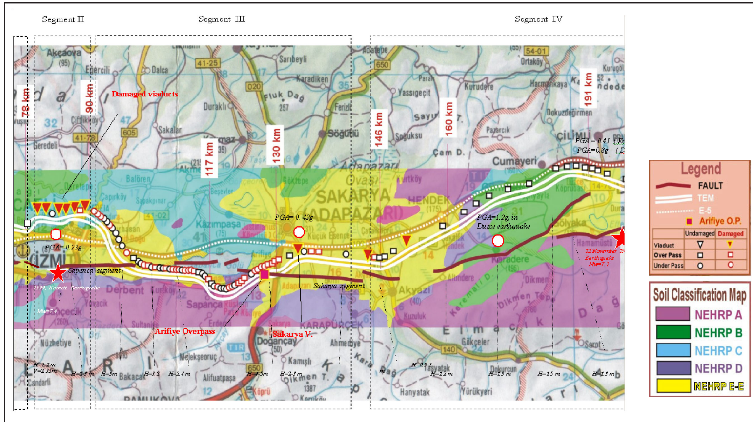
Figure 13 Damage distribution overlaid on a soil classification map (segmented).
