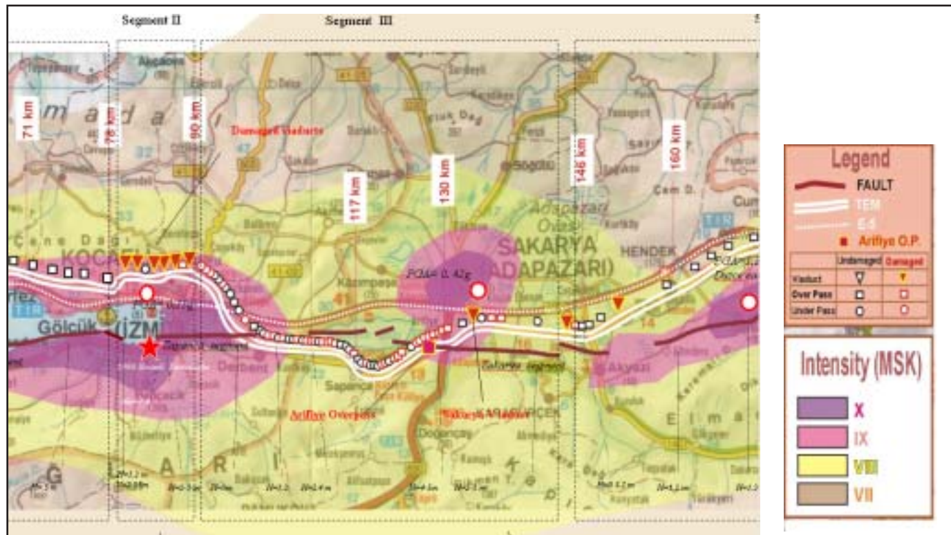
Figure 14 Bridges in TEM segments II and III.
