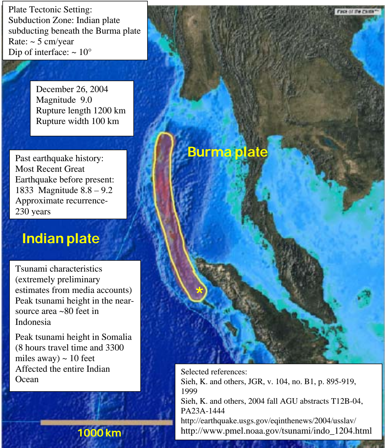
Rupture zone of the December 26 M 9.0 Indonesian earthquake shown in red, epicenter shown by star.
