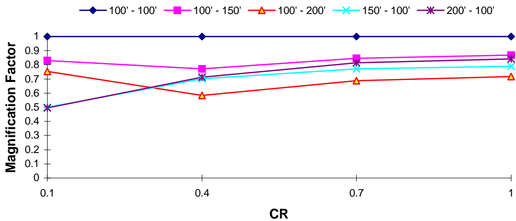
DOF 1 Magnification Factor : Northridge EQ T_1 = 0.5 s, TR = 1.0
