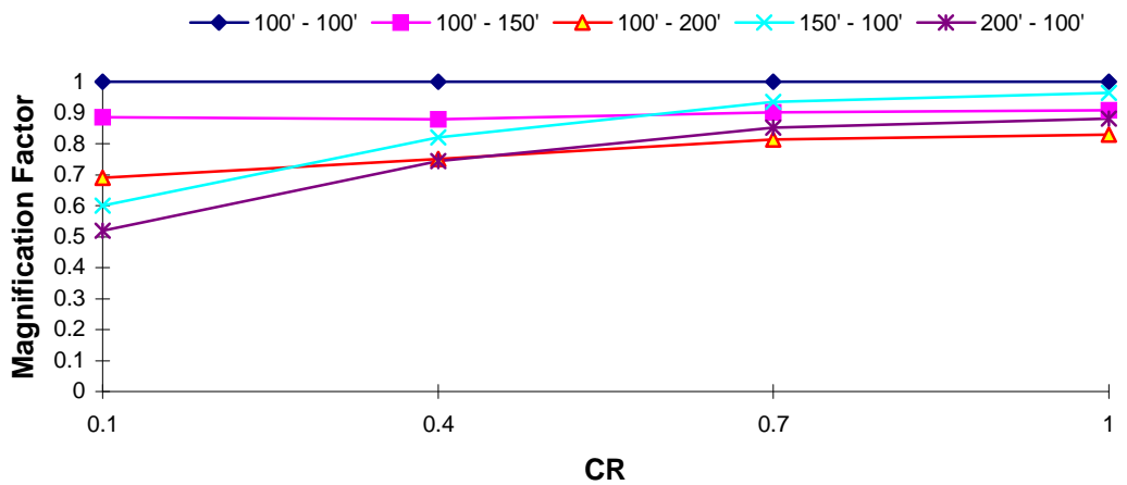
DOF 1 Magnification Factor : Northridge EQ T_1 = 0.5 \text{ s} , TR = 0.7
