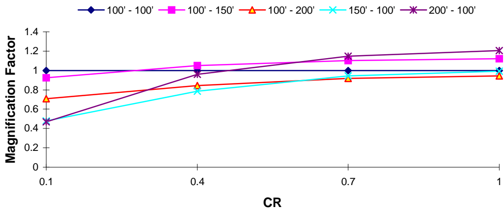
DOF 1 Magnification Factor : El Centro EQ T_1 = 0.5 s, T_R = 0.7
