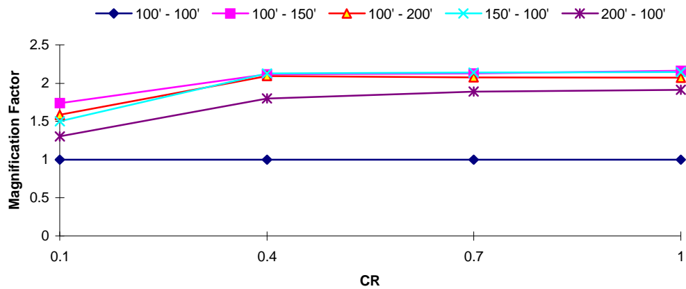
DOF 2 Magnification Factor : Taft EQ T_1 = 0.5 s, TR = 0.1
