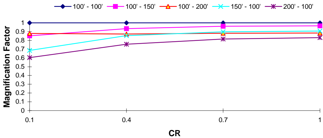
DOF 2 Magnification Factor : Northridge EQ T_1 = 0.5 s, T_R = 0.7
