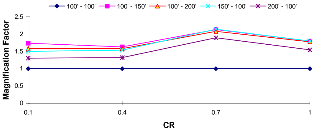
DOF 2 Magnification Factor : Taft EQ T_1 = 0.5 s, TR = 0.4
