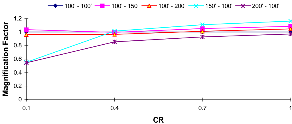
DOF 1 Magnification Factor : Taft EQ T_1 = 0.5 s, T_R = 0.7
