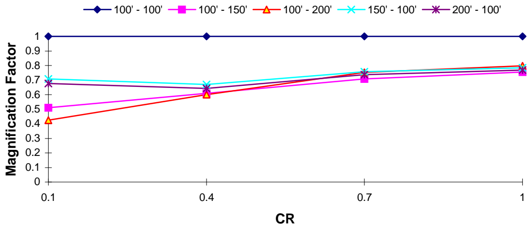
DOF 2 Magnification Factor : Taft EQ T_1 = 0.5 s, TR = 10
