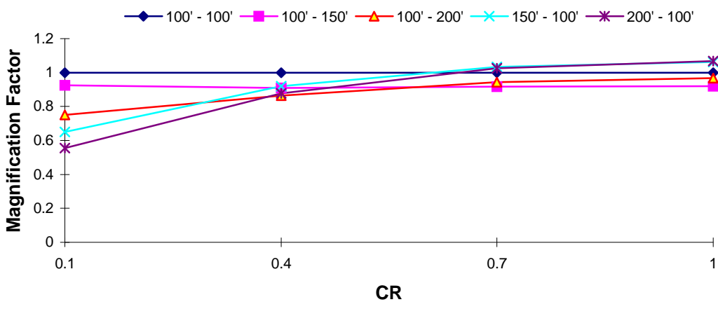
DOF 1 Magnification Factor : Northridge EQ T_1 = 0.5 s, TR = 0.4
