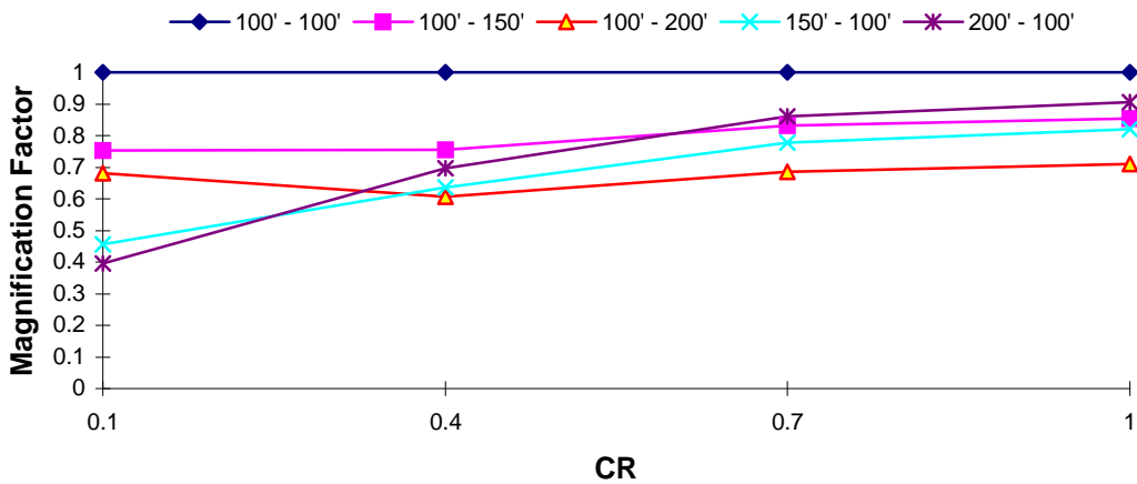
DOF 1 Magnification Factor : El Centro EQ T_1 = 0.5 s, TR = 1.0
