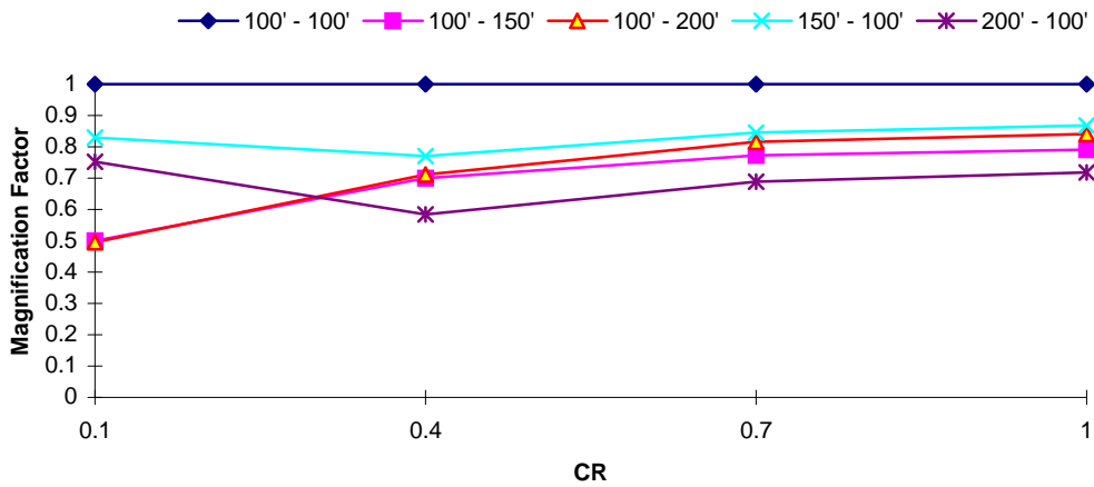
DOF 2 Magnification Factor : Northridge EQ T_1 = 0.5 \text{ s} , TR = 1.0
