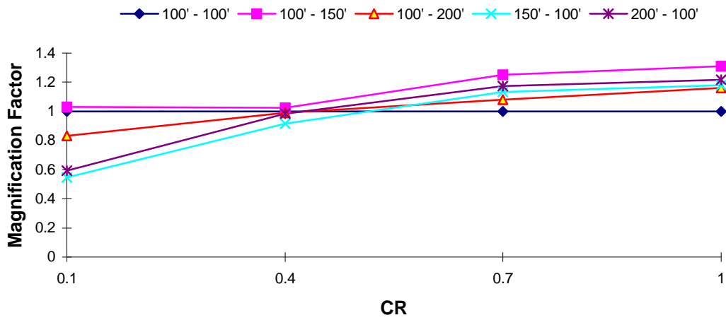
DOF 1 Magnification Factor : El Centro EQ T_1 = 0.5 \text{ s}, TR = 0.4
