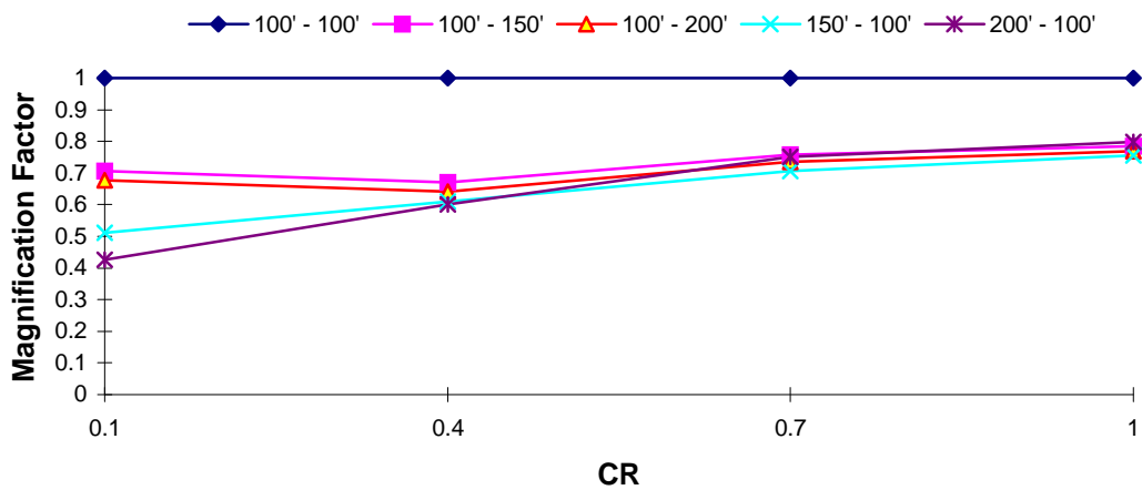
DOF 1 Magnification Factor : Taft EQ T_1 = 0.5 s, T_R = 1.0
