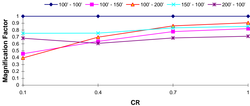
DOF 2 Magnification Factor : El Centro EQ T_1 = 0.5 s, TR = 1.0
