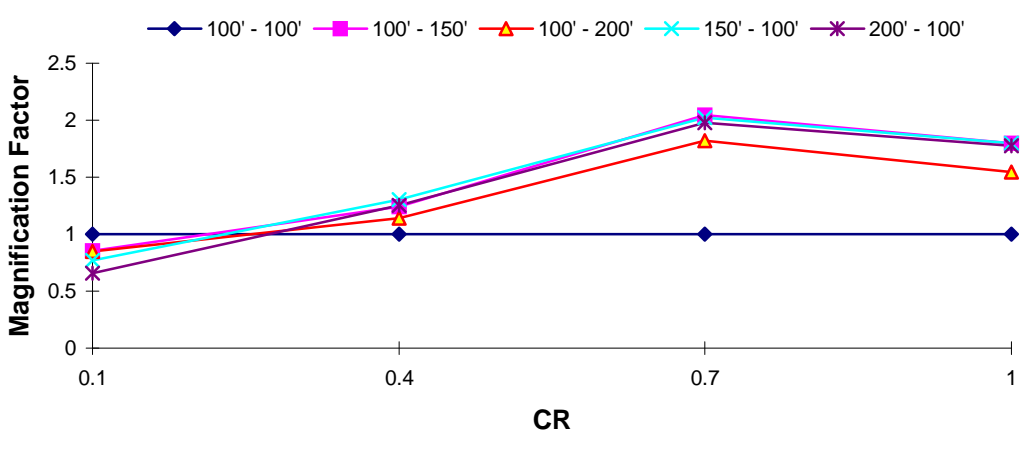
DOF 1 Magnification Factor : Taft EQ T_1 = 0.5 s, TR = 0.4
