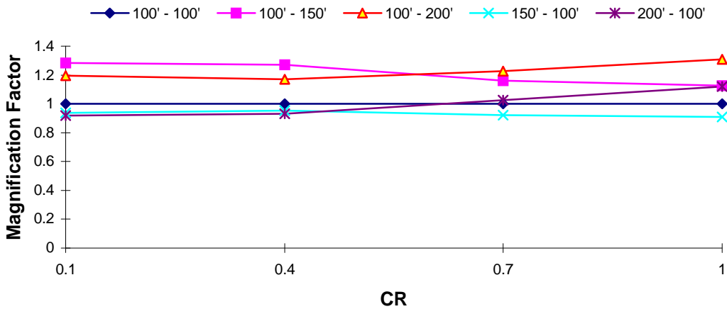
DOF 2 Magnification Factor : Northridge EQ T_1 = 0.5 s, TR = 0.1
