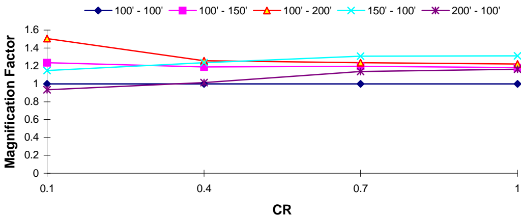
DOF 2 Magnification Factor : El Centro EQ T_1 = 0.5 s, TR = 0.4
