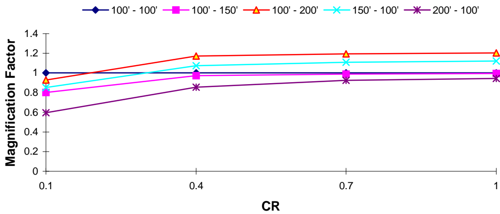
DOF 2 Magnification Factor : El Centro EQ T_1 = 0.5 s, T_R = 0.7
