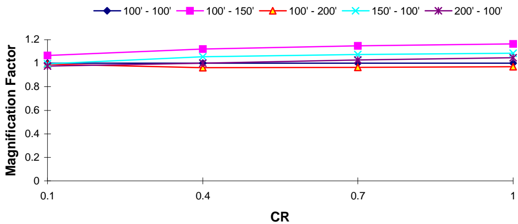
DOF 2 Magnification Factor : Taft EQ T_1 = 0.5 s, TR = 0.7
