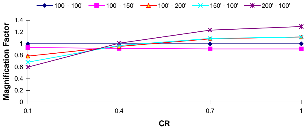
DOF 1 Magnification Factor : Northridge EQ T_1 = 0.5 \text{ s}, TR = 0.1
