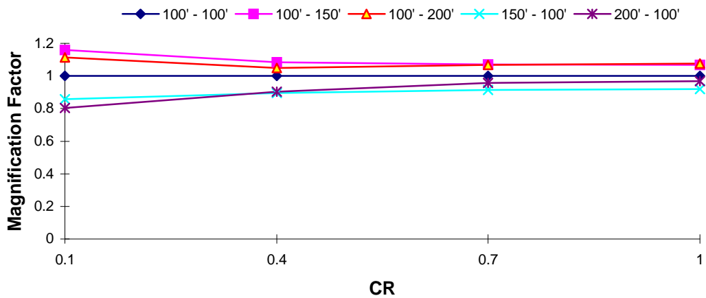
DOF 2 Magnification Factor : Northridge EQ T_1 = 0.5 s, T_R = 0.4
