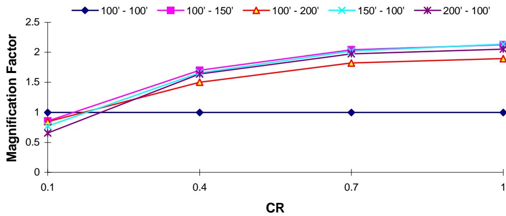
DOF 1 Magnification Factor : Taft EQ T_1 = 0.5 s, T_R = 0.1
