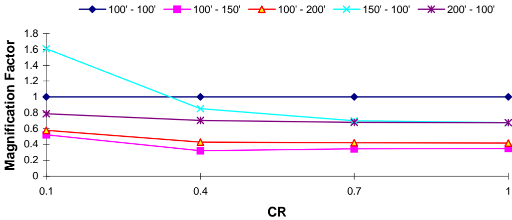
DOF 2 Magnification Factor : El Centro EQ T_1 = 1.0 s, TR = 0.1
