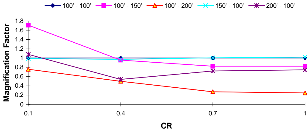
DOF 2 Magnification Factor : Taft EQ T_1 = 1.0 s, TR = 1.0
