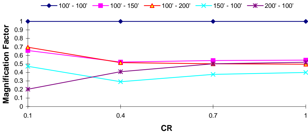
DOF 1 Magnification Factor : Taft EQ T_1 = 1.0 s, TR = 0.1
