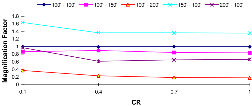
DOF 2 Magnification Factor : El Centro EQ T_1 = 1.0 s, TR = 0.7
