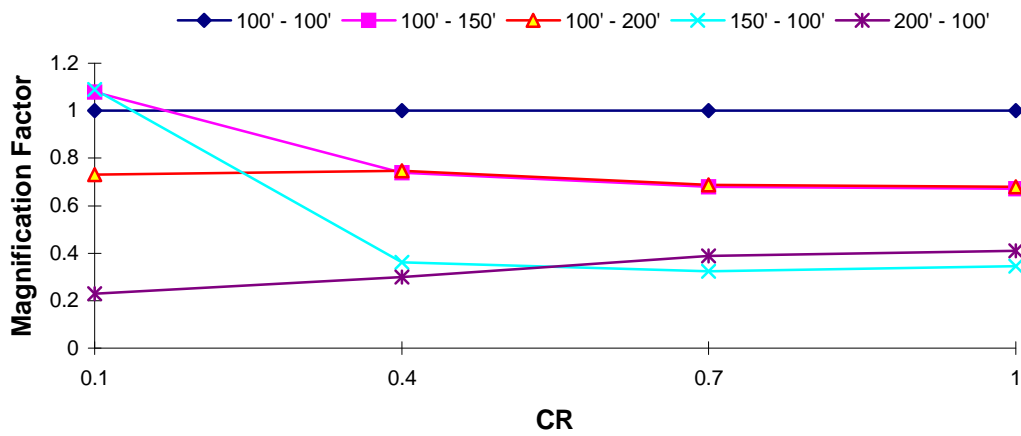
DOF 1 Magnification Factor : El Centro EQ T_1 = 1.0 s, T_R = 0.1
