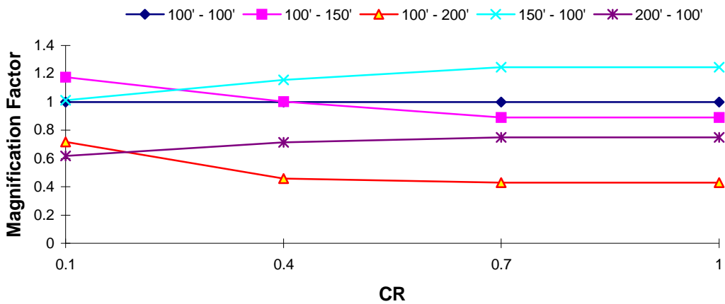
DOF 2 Magnification Factor : Northridge EQ T_1 = 1.0 s, T_R = 1.0
