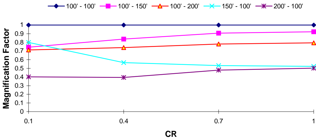
DOF 1 Magnification Factor : Northridge EQ T_1 = 1.0 s, T_R = 0.7
