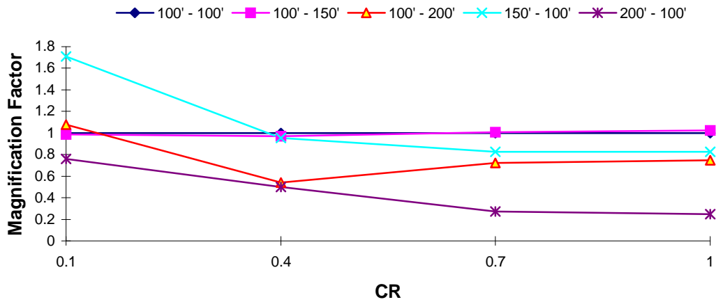
DOF 1 Magnification Factor : Taft EQ T_1 = 1.0 s, TR = 1.0
