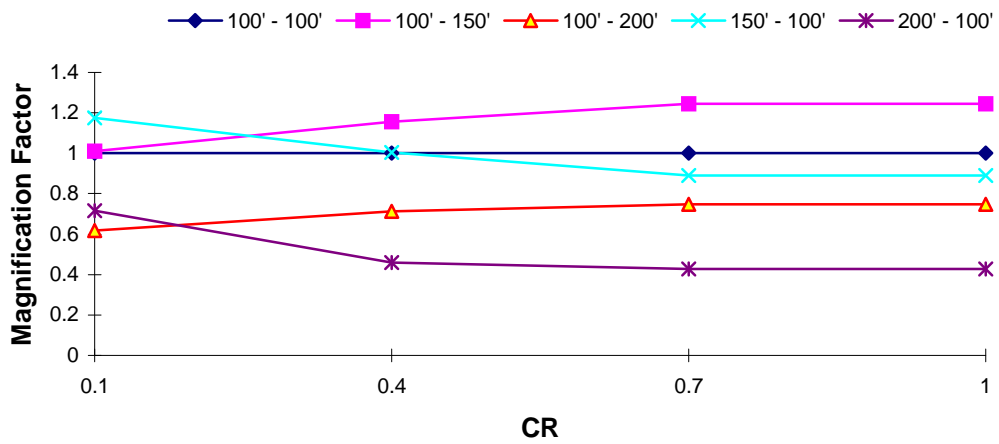
DOF 1 Magnification Factor : Northridge EQ T_1 = 1.0 s, TR = 1.0
