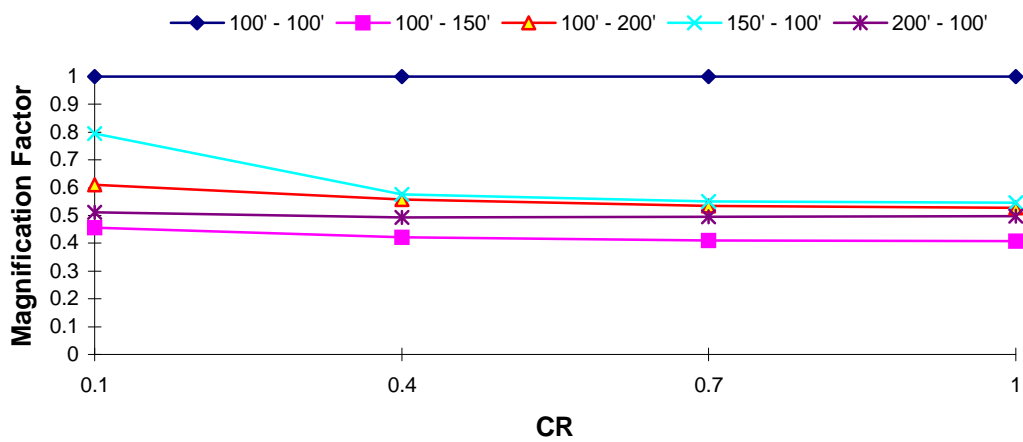
DOF 2 Magnification Factor : Taft EQ T_1 = 1.0 s, TR = 0.1
