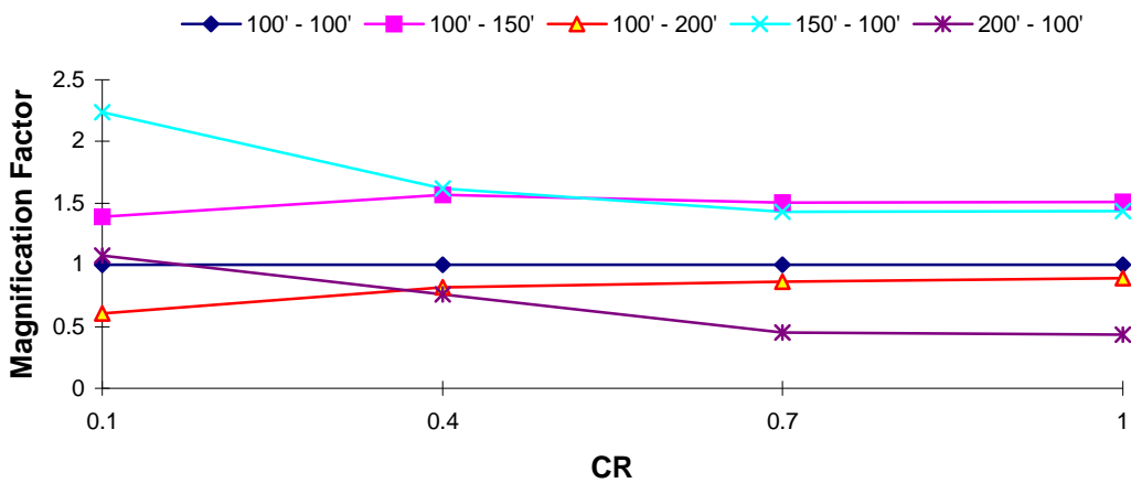
DOF 1 Magnification Factor : El Centro EQ T_1 = 1.0 s, T_R = 1.0
