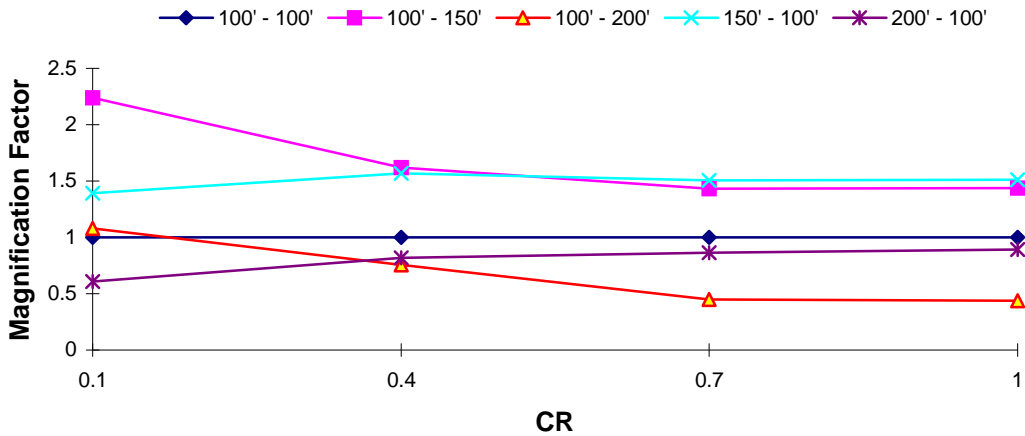
DOF 2 Magnification Factor : El Centro EQ T_1 = 1.0 s, T_R = 1.0
