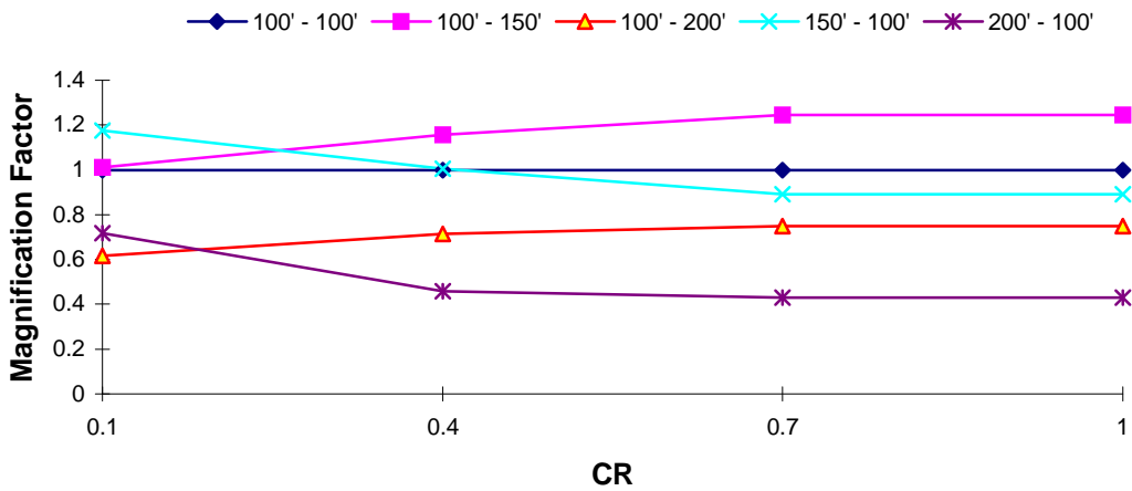
DOF 1 Magnification Factor : Northridge EQ T_1 = 1.0 s, T_R = 0.1
