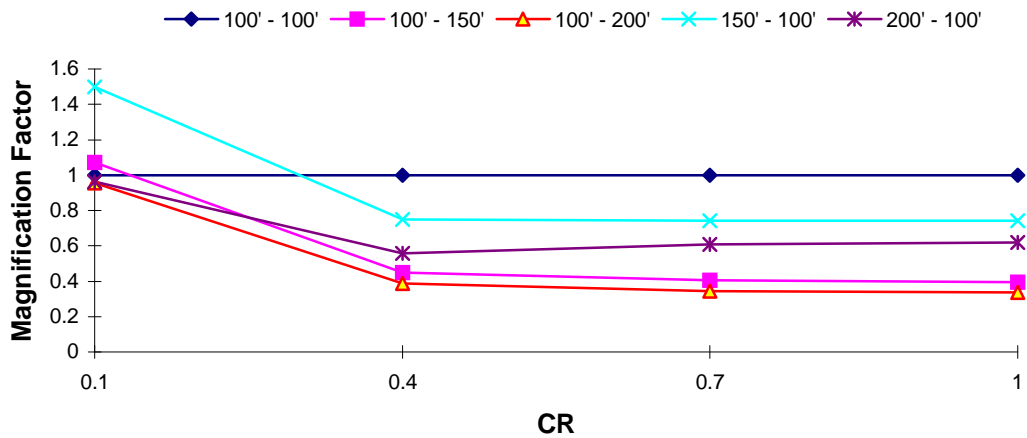
DOF 2 Magnification Factor : Taft EQ T 1 = 1.0 s, TR = 0.7
