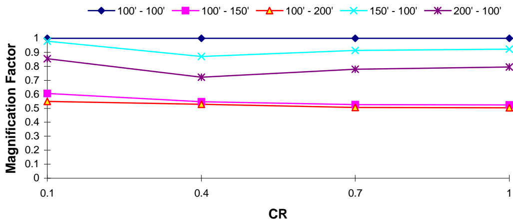
DOF 2 Magnification Factor : Northridge EQ T_1 = 1.0 s, T_R = 0.7
