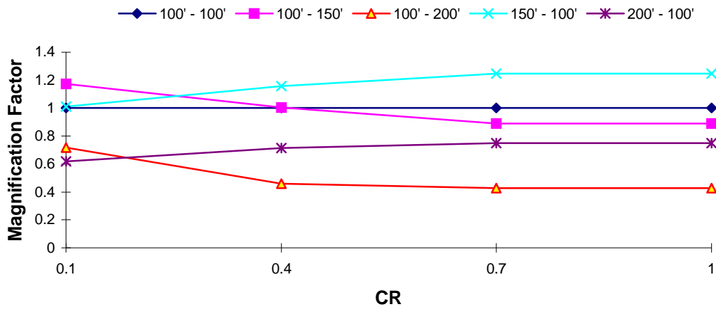
DOF 2 Magnification Factor : Northridge EQ T_1 = 1.0 s, T_R = 0.1
