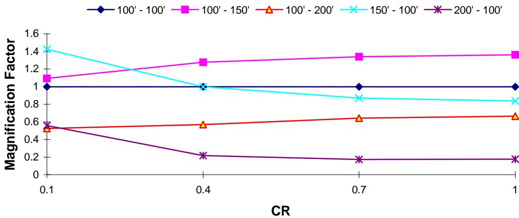
DOF 1 Magnification Factor : El Centro EQ T_1 = 1.0 s, T_R = 0.7
