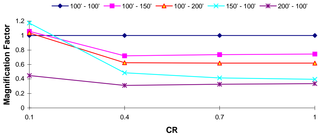
DOF 1 Magnification Factor : Taft EQ T_1 = 1.0 s, TR = 0.7
