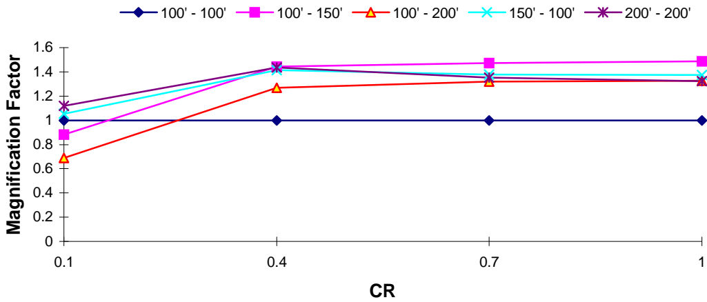
DOF 1 Magnification Factor : Northridge EQ T_1 = 1.5 s, TR = 0.4
