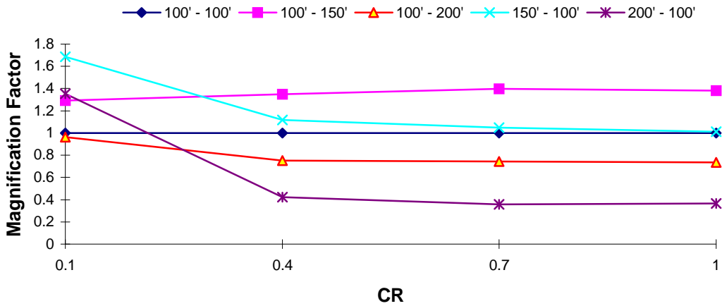
DOF 1 Magnification Factor : Northridge EQ T_1 = 1.5 s, TR = 0.1
