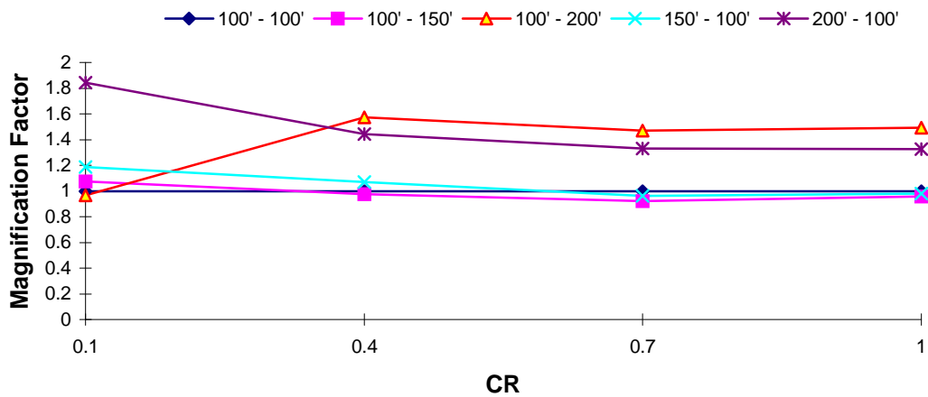
DOF 1 Magnification Factor : Taft EQ T 1 = 1.5 s, TR = 1.0
