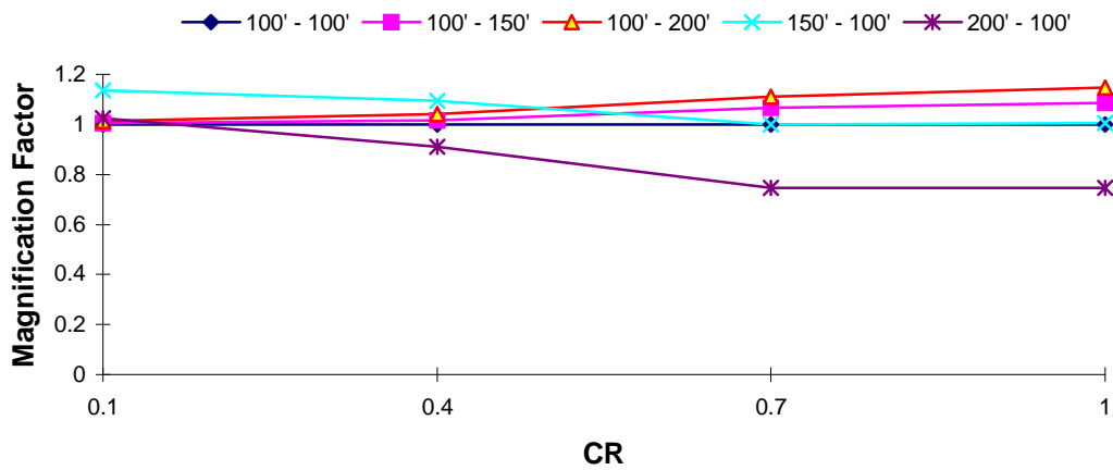
DOF 1 Magnification Factor : El Centro EQ T_1 = 1.5 s, TR = 1.0
