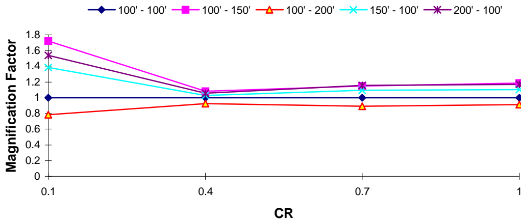
DOF 1 Magnification Factor : Northridge EQ T_1 = 1.5 s, T_R = 0.7
