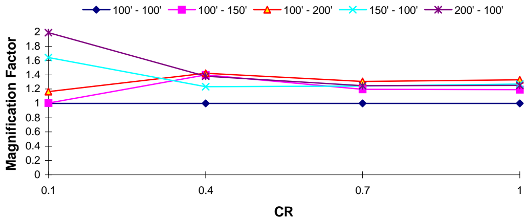
DOF 1 Magnification Factor : Northridge EQ T_1 = 1.5 s, TR = 1.0
