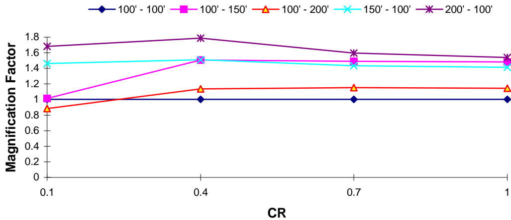
DOF 2 Magnification Factor : Taft EQ T_1 = 1.5 s, TR = 0.4
