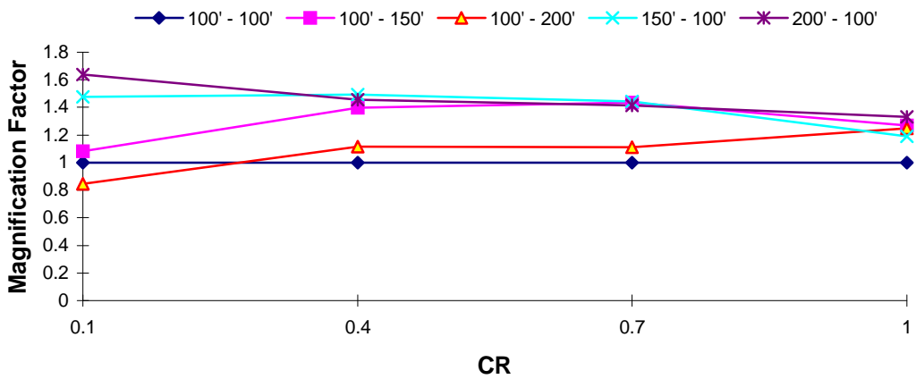
DOF 2 Magnification Factor : Northridge EQ T_1 = 1.5 s, TR = 0.7
