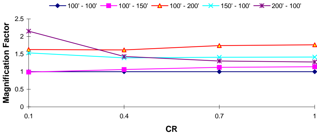
DOF 1 Magnification Factor : Taft EQ T_1 = 1.5 s, TR = 0.7
