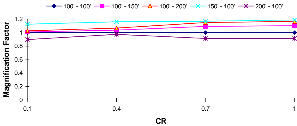
DOF 1 Magnification Factor : El Centro EQ T_1 = 1.5 s, T_R = 0.7
