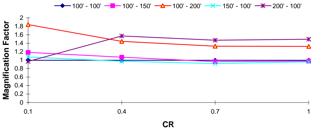
DOF 2 Magnification Factor : Taft EQ T_1 = 1.5 s, TR = 1.0
