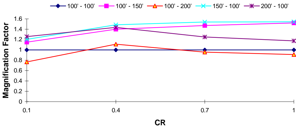
DOF 2 Magnification Factor : El Centro EQ T_1 = 1.5 s, TR = 0.1
