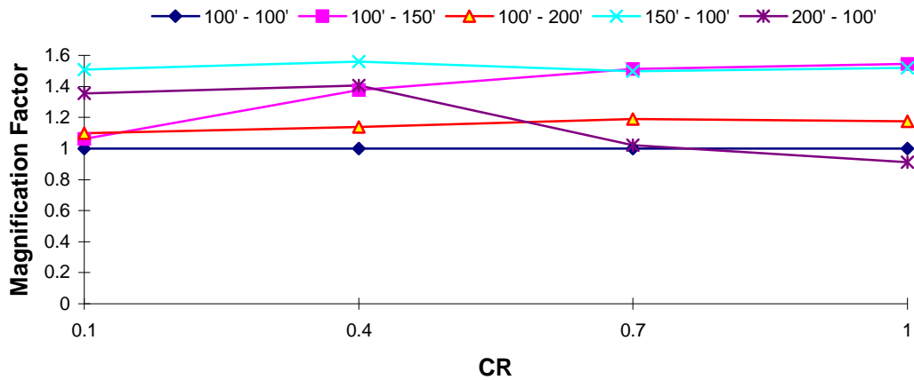
DOF 1 Magnification Factor : El Centro EQ T_1 = 1.5 s, TR = 0.1
