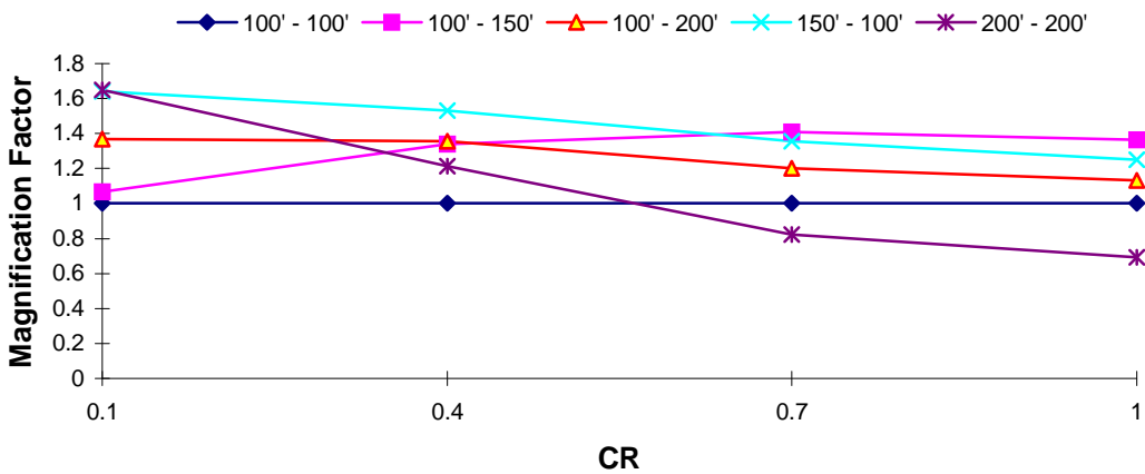
DOF 2 Magnification Factor : Northridge EQ T_1 = 1.5 s, TR = 0.1
