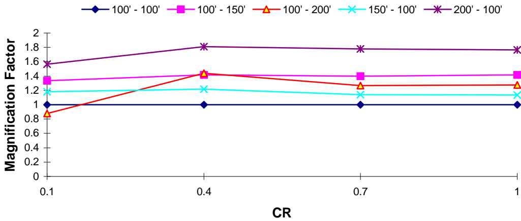
DOF 2 Magnification Factor : Taft EQ T_1 = 1.5 s, T_R = 0.7
