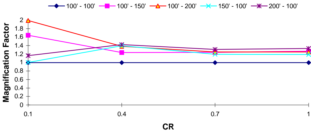
DOF 2 Magnification Factor : Northridge EQ T_1 = 1.5 s, TR = 1.0
