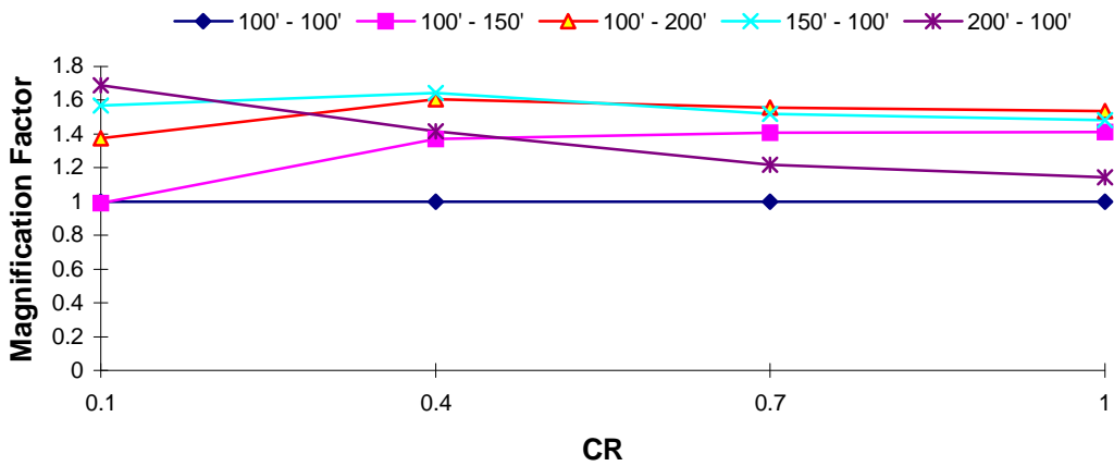
DOF 1 Magnification Factor : Taft EQ T_1 = 1.5 s, TR = 0.4
