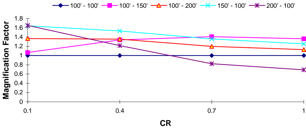
DOF 1 Magnification Factor : Taft EQ T_1 = 1.5 s, TR = 0.1
