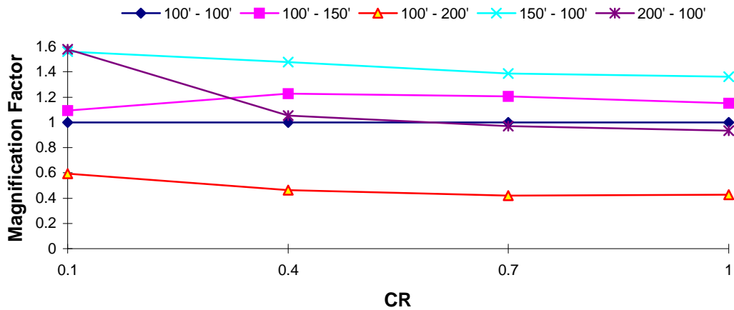
DOF 2 Magnification Factor : Northridge EQ T_1 = 1.5 \text{ s}, TR = 0.4
