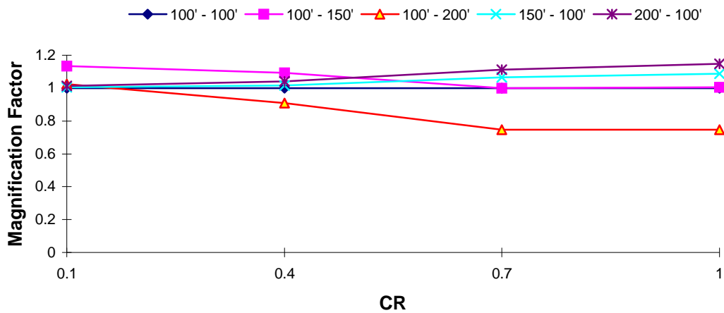
DOF 2 Magnification Factor : El Centro EQ T_1 = 1.5 s, TR = 1.0
