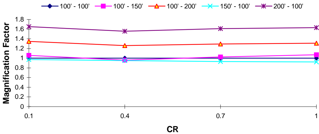
DOF 2 Magnification Factor : Taft EQ T_1 = 2.0 s, TR = 0.1
