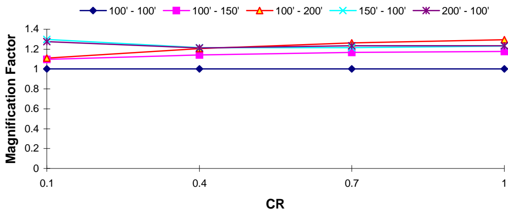
DOF 1 Magnification Factor : Northridge EQ T_1 = 2.0 s, T_R = 0.4
