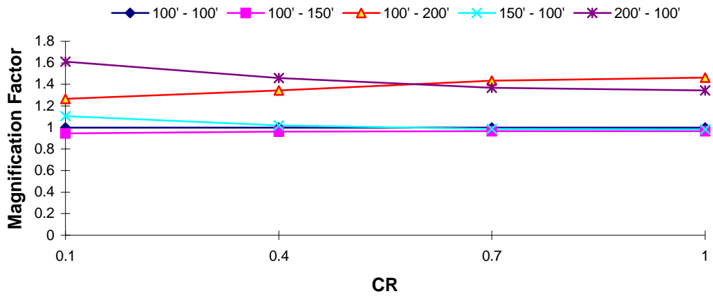
DOF 1 Magnification Factor : Taft EQ T_1 = 2.0 s, TR = 0.4
