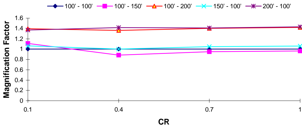
DOF 1 Magnification Factor : Taft EQ T_1 = 2.0 s, TR = 0.7
