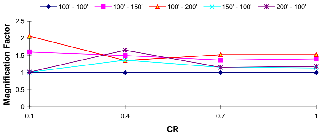
DOF 2 Magnification Factor : Northridge EQ T_1 = 2.0 s, TR = 1.0
