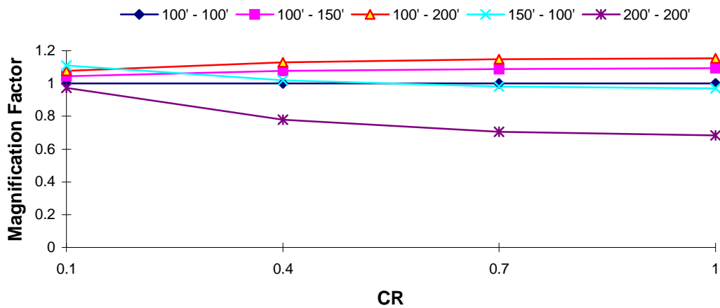
DOF 1 Magnification Factor : El Centro EQ T_1 = 2.0 s, TR = 0.1
