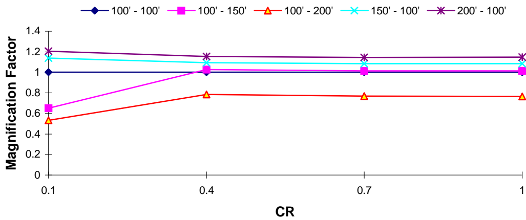
DOF 2 Magnification Factor : El Centro EQ T_1 = 2.0 s, TR = 0.4
