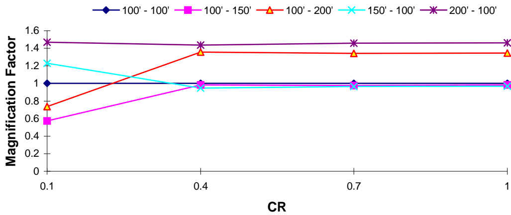
DOF 2 Magnification Factor : Taft EQ T_1 = 2.0 s, TR = 0.4
