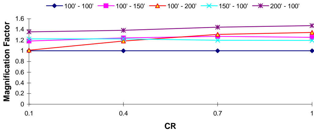
DOF 2 Magnification Factor : Northridge EQ T_1 = 2.0 s, TR = 0.1
