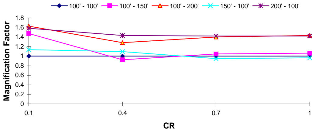
DOF 2 Magnification Factor : Taft EQ T_1 = 2.0 s, TR = 0.7
