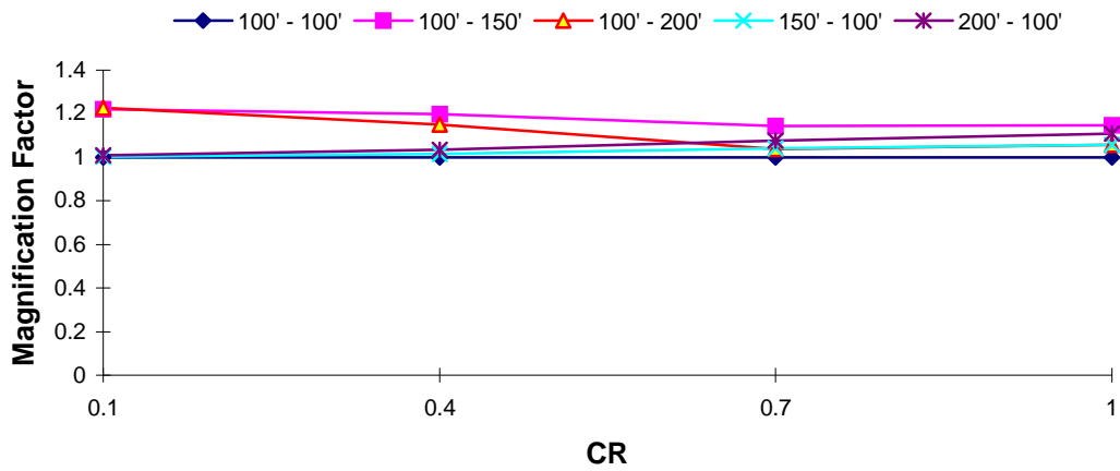
DOF 2 Magnification Factor : El Centro EQ T_1 = 2.0 s, TR = 1.0
