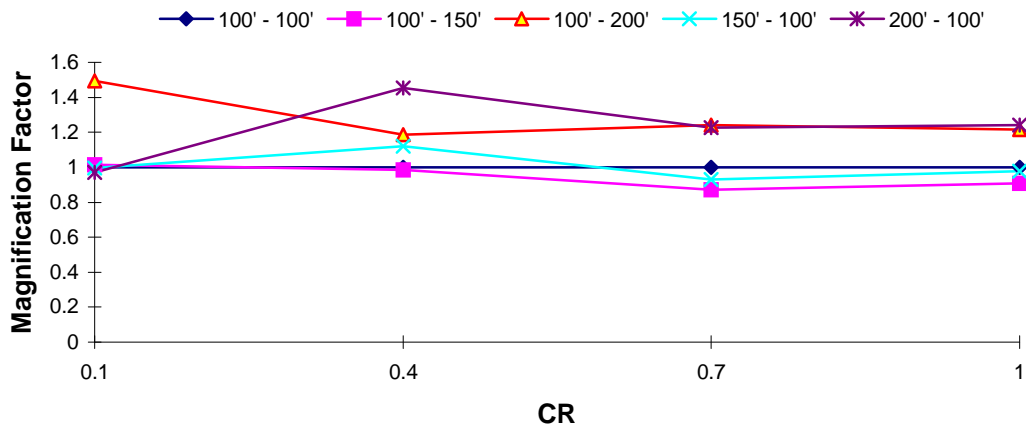
DOF 2 Magnification Factor : Taft EQ T_1 = 2.0 s, TR = 1.0
