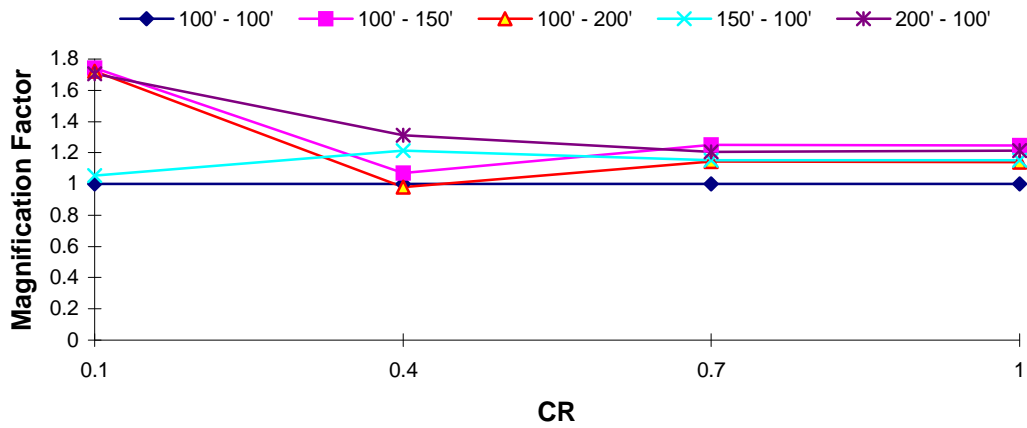
DOF 2 Magnification Factor : Northridge EQ T_1 = 2.0 s, T_R = 0.7
