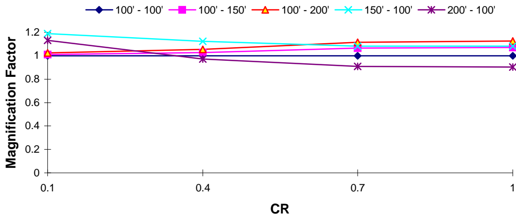
DOF 1 Magnification Factor : El Centro EQ T_1 = 2.0 s, TR = 0.7
