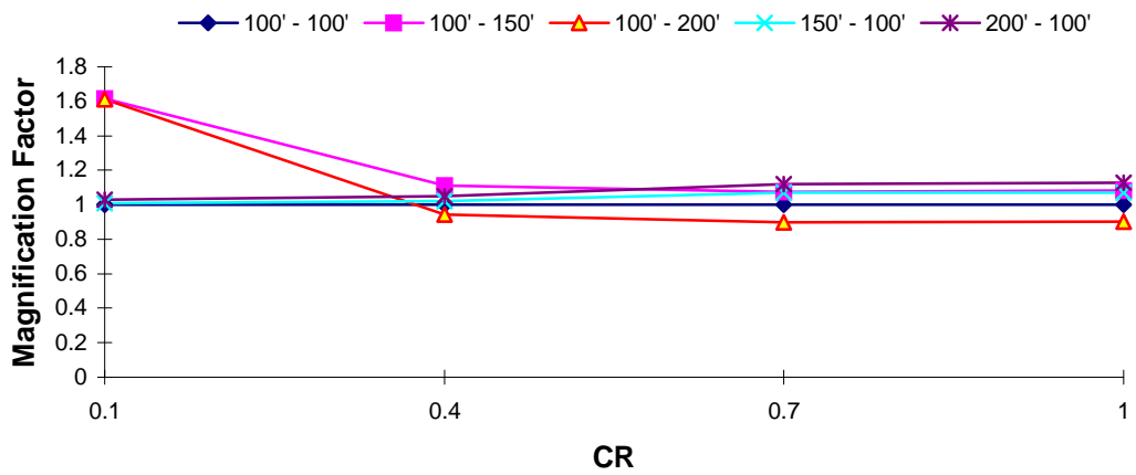
DOF 2 Magnification Factor : El Centro EQ T_1 = 2.0 s, T_R = 0.7
