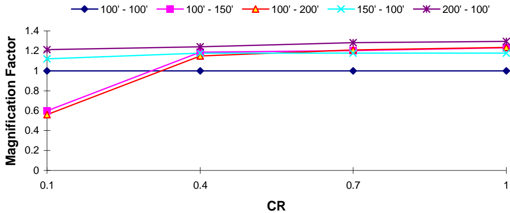
DOF 2 Magnification Factor : Northridge EQ T_1 = 2.0 s, TR = 0.4
