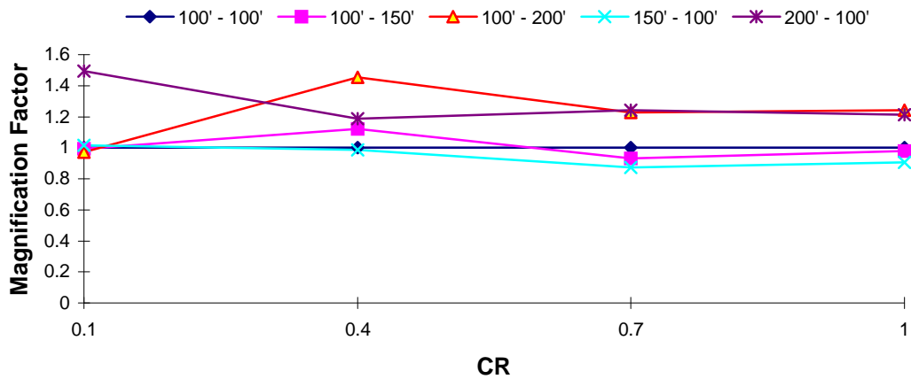
DOF 1 Magnification Factor : Taft EQ T_1 = 2.0 s, TR = 1.0
