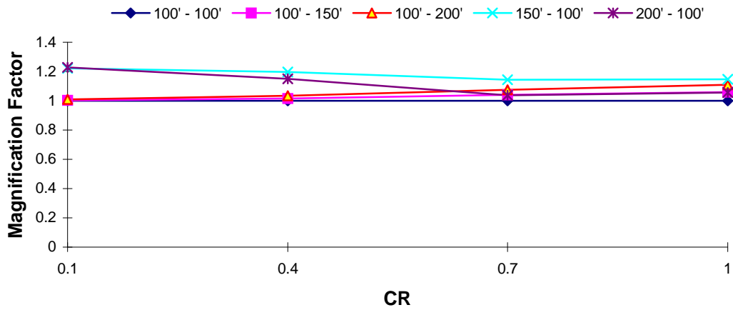
DOF 1 Magnification Factor : El Centro EQ T_1 = 2.0 s, TR = 1.0
