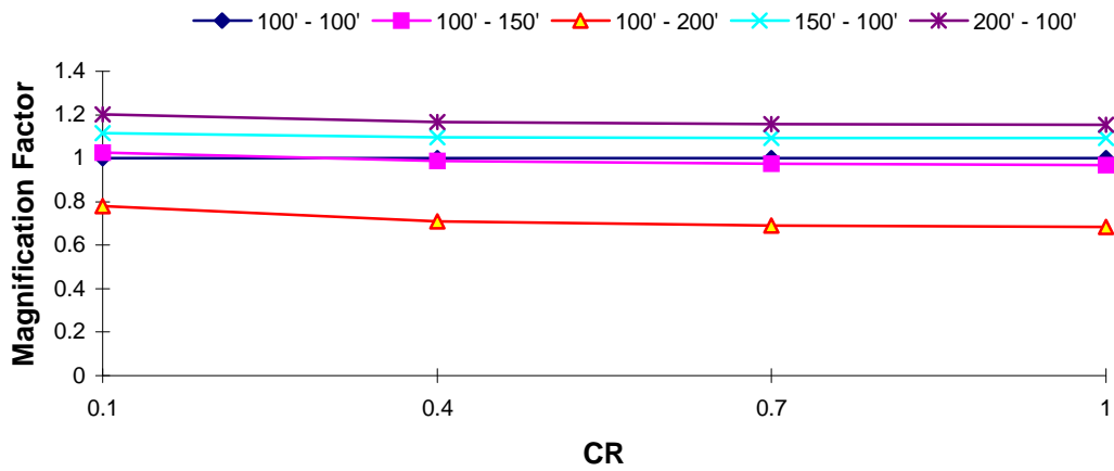
DOF 2 Magnification Factor : El Centro EQ T_1 = 2.0 s, TR = 0.1
