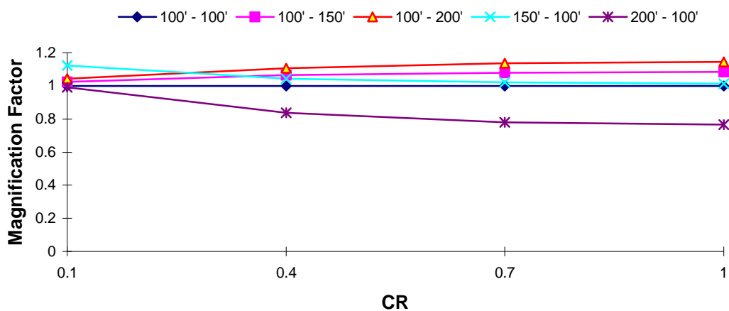
DOF 1 Magnification Factor : El Centro EQ T_1 = 2.0 s, TR = 0.4
