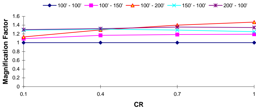
DOF 1 Magnification Factor : Northridge EQ T_1 = 2.0 s, TR = 0.1
