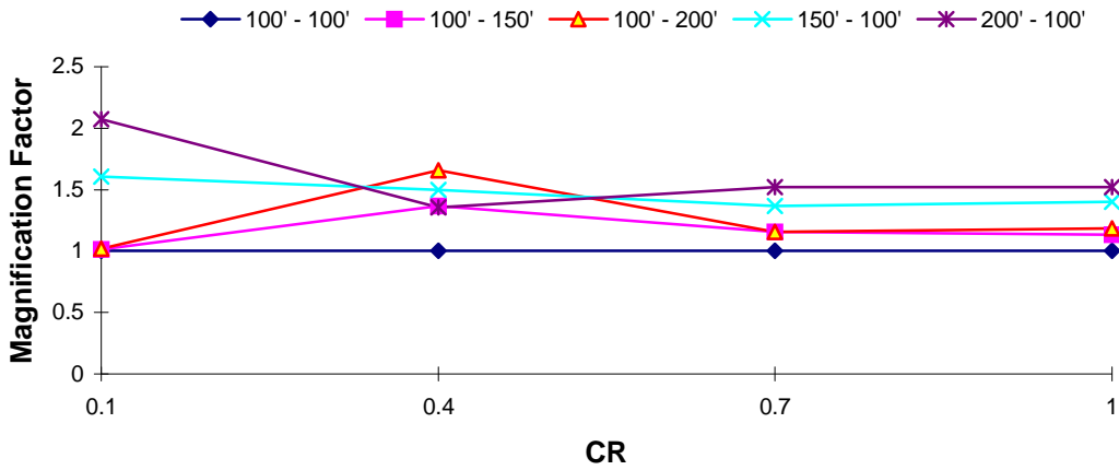
DOF 1 Magnification Factor : Northridge EQ T_1 = 2.0 s, T_R = 1.0
