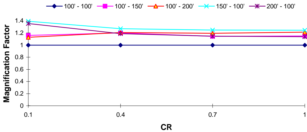
DOF 1 Magnification Factor : Northridge EQ T 1 = 2.0 s, TR = 0.7
