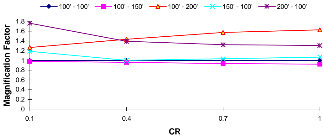
DOF 1 Magnification Factor : Taft EQ T_1 = 2.0 s, TR = 0.1
