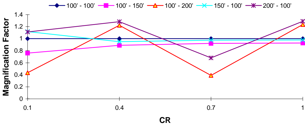
DOF 2 Magnification Factor : Taft EQ T_1 = 2.5 s, TR = 0.4
