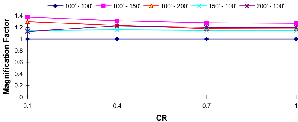
DOF 2 Magnification Factor : Northridge EQ T_1 = 2.5 s, TR = 0.1
