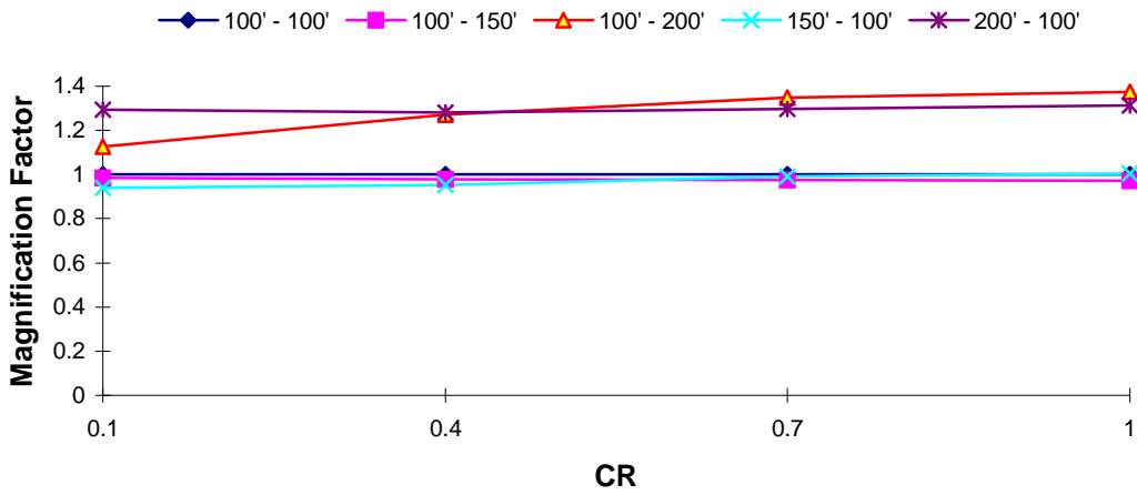
DOF 1 Magnification Factor : Taft EQ T_1 = 2.5 s, TR = 0.1
