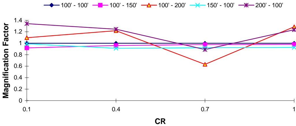
DOF 1 Magnification Factor : Taft EQ T_1 = 2.5 s, TR = 0.4
