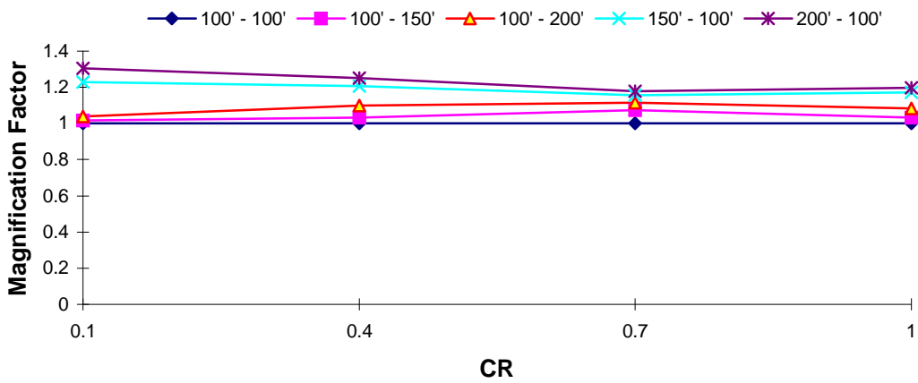
DOF 1 Magnification Factor : El Centro EQ T_1 = 2.5 s, TR = 1.0
