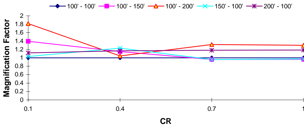
DOF 2 Magnification Factor : Taft EQ T_1 = 2.5 s, TR = 0.7
