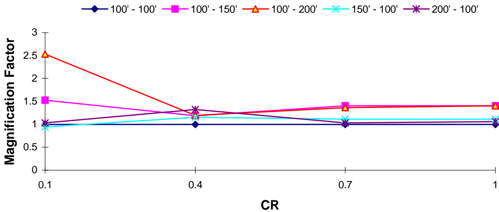
DOF 2 Magnification Factor : Northridge EQ T_1 = 2.5 s, T_R = 0.7
