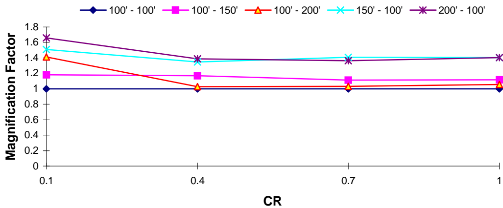
DOF 1 Magnification Factor : Northridge EQ T_1 = 2.5 s, T_R = 0.7
