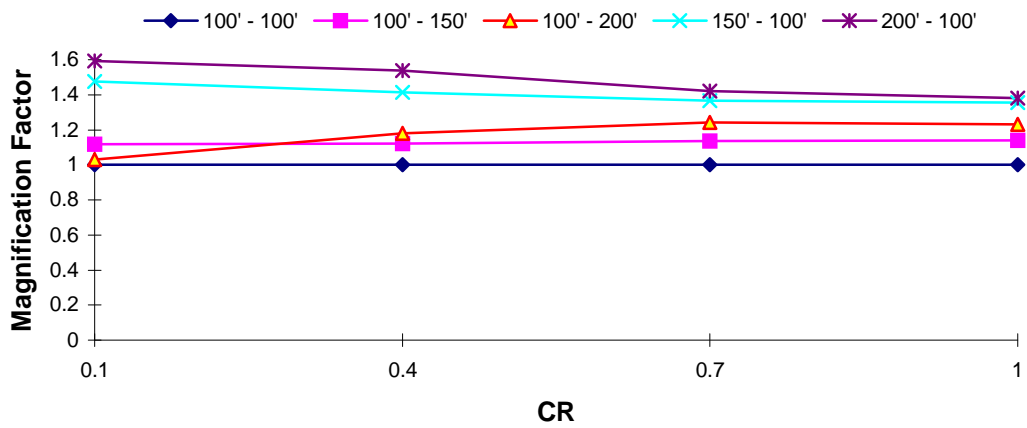
DOF 1 Magnification Factor : Northridge EQ T_1 = 2.5 s, T_R = 0.4
