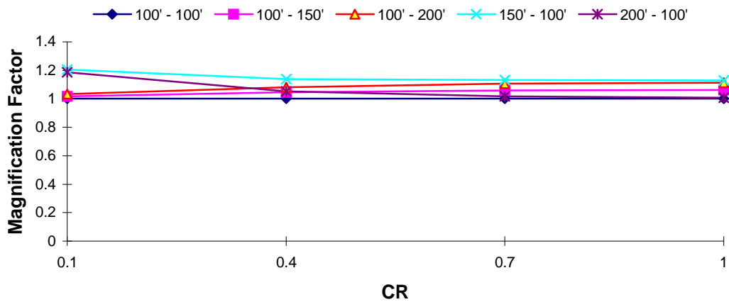
DOF 1 Magnification Factor : El Centro EQ T_1 = 2.5 s, TR = 0.4
