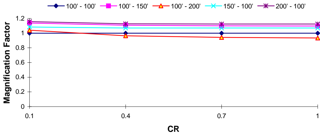
DOF 2 Magnification Factor : El Centro EQ T_1 = 2.5 s, TR = 0.1
