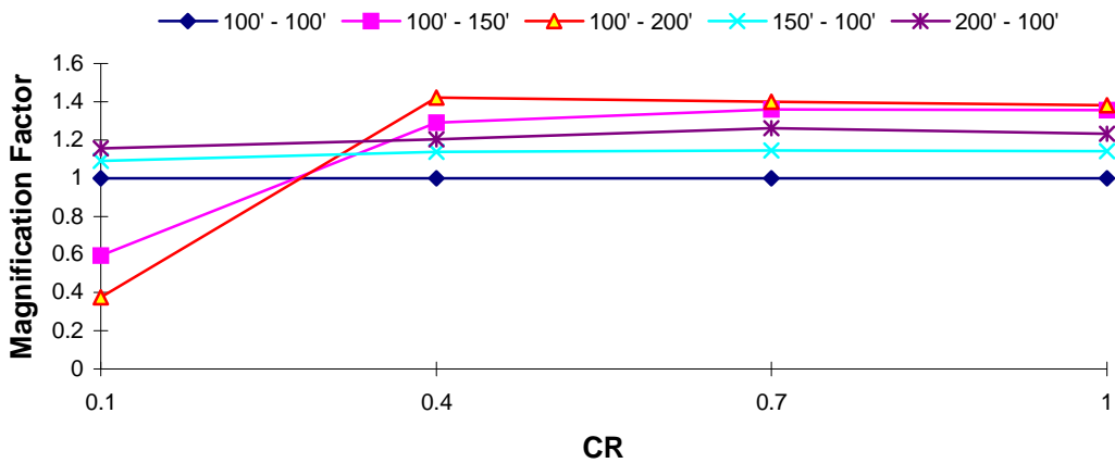
DOF 2 Magnification Factor : Northridge EQ T_1 = 2.5 s, TR = 0.4
