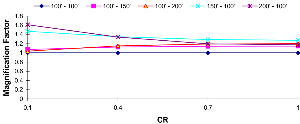
DOF 1 Magnification Factor : Northridge EQ T_1 = 2.5 s, TR = 0.1
