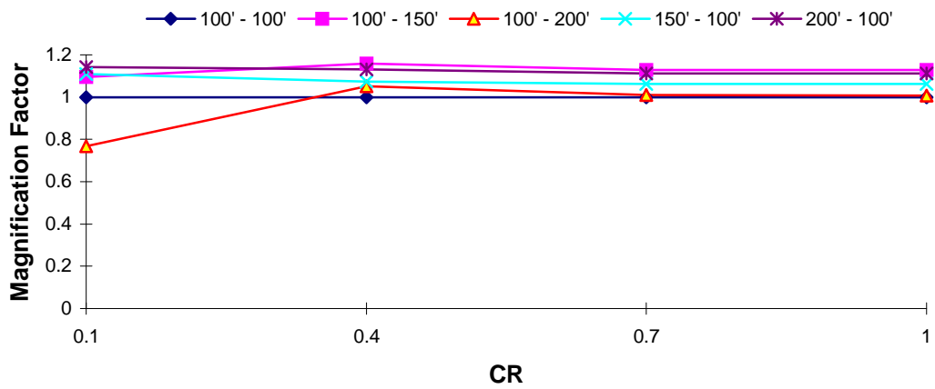
DOF 2 Magnification Factor : El Centro EQ T_1 = 2.5 s, TR = 0.4
