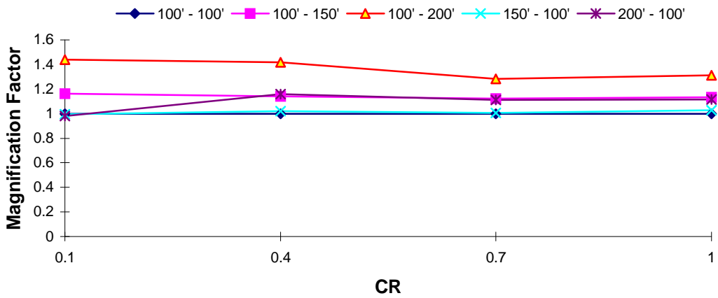
DOF 2 Magnification Factor : Taft EQ T 1 = 2.5 s, TR = 1.0
