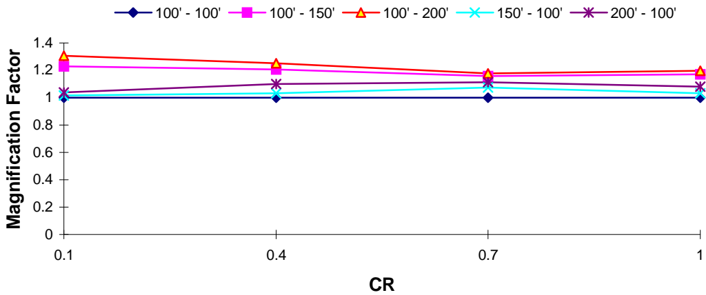
DOF 2 Magnification Factor : El Centro EQ T_1 = 2.5 s, TR = 1.0
