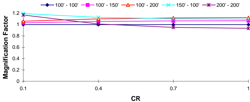
DOF 1 Magnification Factor : El Centro EQ T_1 = 2.5 s, TR = 0.1
