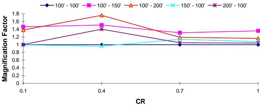
DOF 2 Magnification Factor : Northridge EQ T_1 = 2.5 s, TR = 1.0
