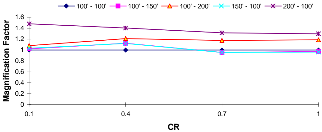
DOF 1 Magnification Factor : Taft EQ T_1 = 2.5 s, TR = 0.7
