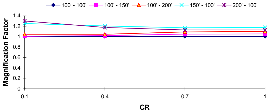
DOF 1 Magnification Factor : El Centro EQ T_1 = 2.5 s, T_R = 0.7
