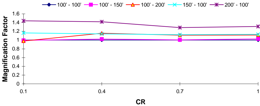
DOF 1 Magnification Factor : Taft EQ T_1 = 2.5 s, TR = 1.0
