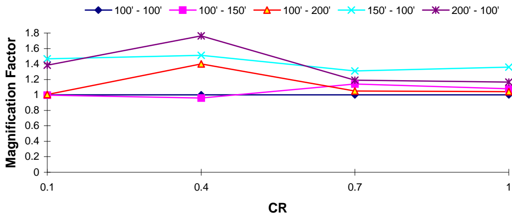
DOF 1 Magnification Factor : Northridge EQ T_1 = 2.5 s, TR = 1.0
