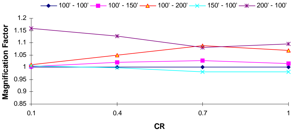
DOF 1 Magnification Factor : El Centro EQ T_1 = 3.0 s, TR = 1.0
