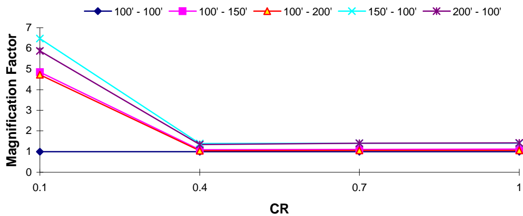
DOF 1 Magnification Factor : Northridge EQ T_1 = 3.0 s, TR = 0.1
