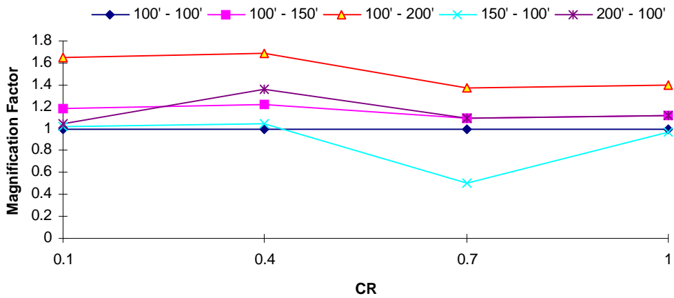
DOF 2 Magnification Factor : Northridge EQ T_1 = 3.0 s, T_R = 1.0
