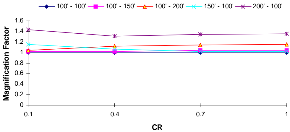
DOF 1 Magnification Factor : Taft EQ T_1 = 3.0 s, T_R = 0.4
