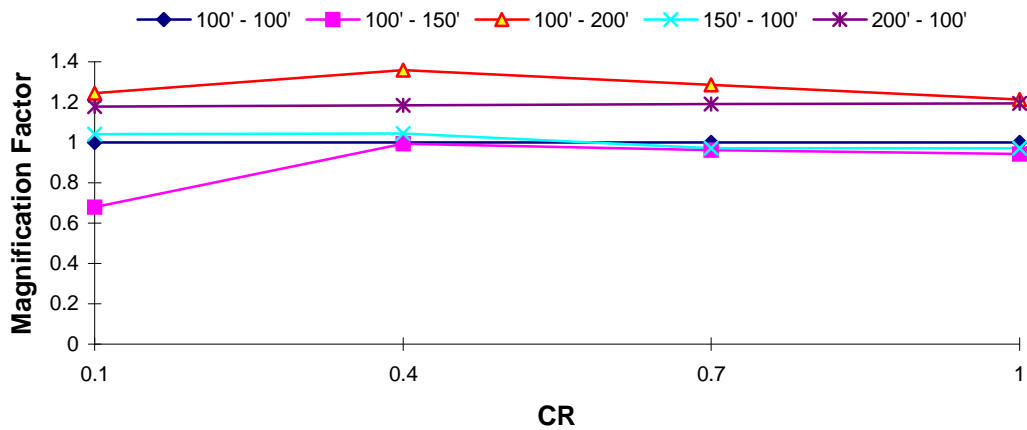
DOF 2 Magnification Factor : Taft EQ T_1 = 3.0 s, TR = 0.1
