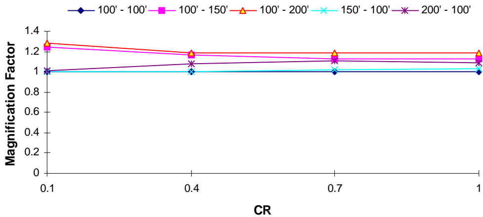
DOF 2 Magnification Factor : El Centro EQ T_1 = 3.0 s, T_R = 0.7
