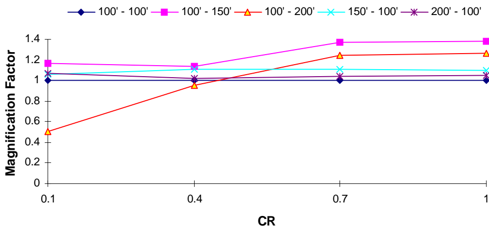
DOF 2 Magnification Factor : Northridge EQ T_1 = 3.0 s, TR = 0.4
