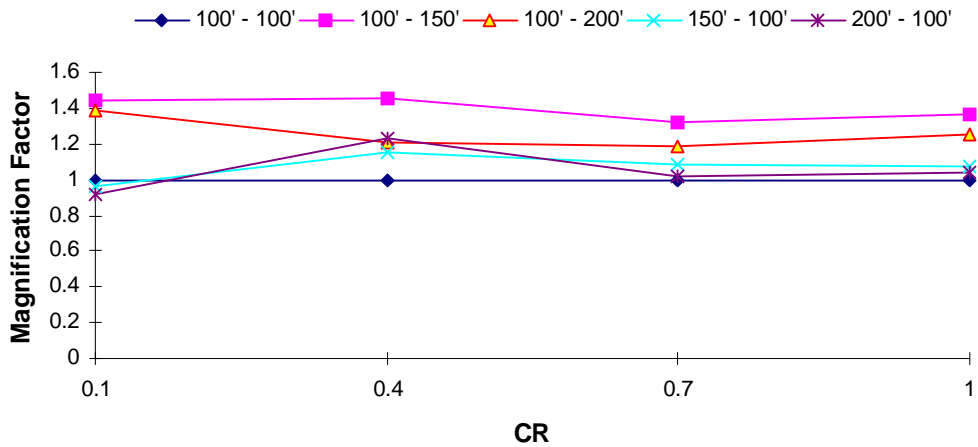
DOF 2 Magnification Factor : Northridge EQ T_1 = 3.0 s, T_R = 0.7
