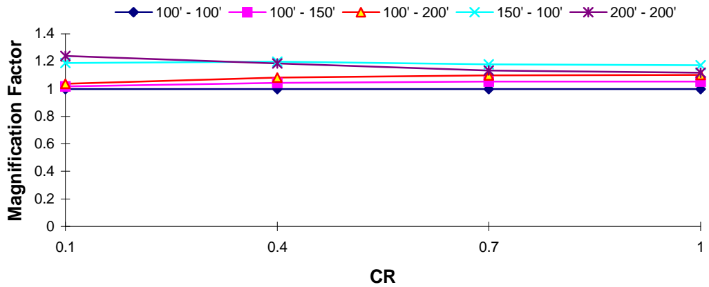
DOF 1 Magnification Factor : El Centro EQ T_1 = 3.0 s, TR = 0.1
