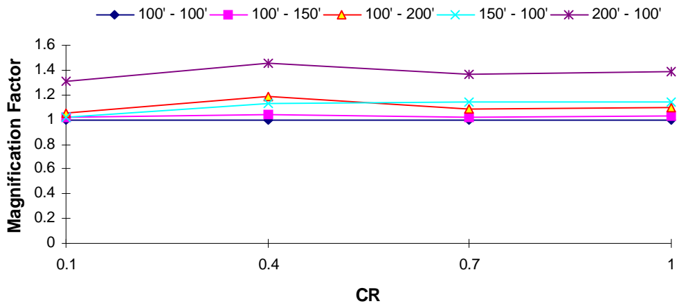
DOF 1 Magnification Factor : Taft EQ T_1 = 3.0 s, T_R = 0.7
