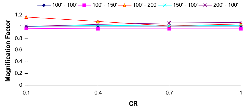
DOF 2 Magnification Factor : Taft EQ T_1 = 3.0 s, TR = 1.0
