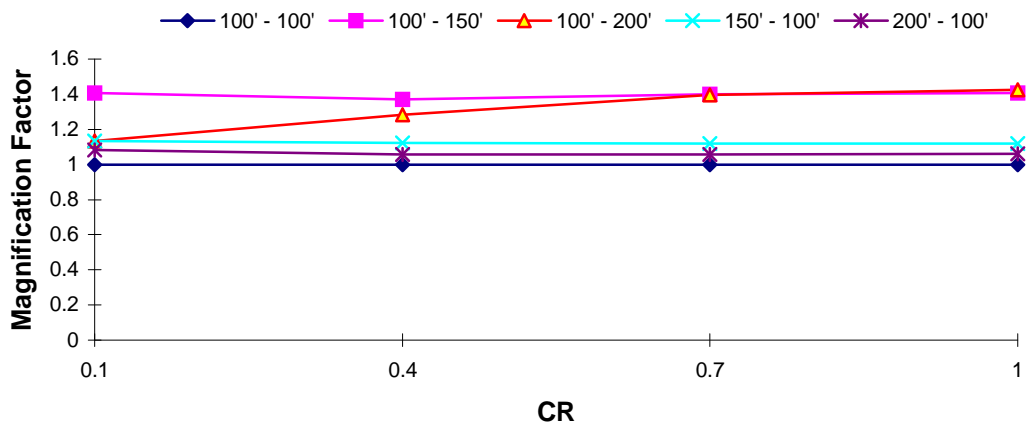
DOF 2 Magnification Factor : Northridge EQ T_1 = 3.0 s, TR = 0.1
