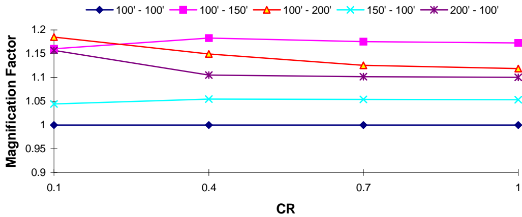
DOF 2 Magnification Factor : El Centro EQ T_1 = 3.0 s, TR = 0.1
