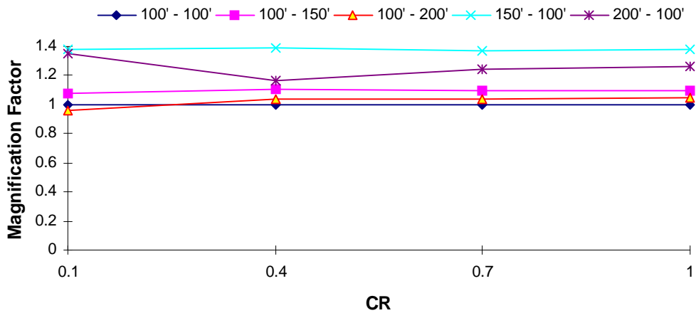
DOF 1 Magnification Factor : Northridge EQ T_1 = 3.0 s, TR = 0.4
