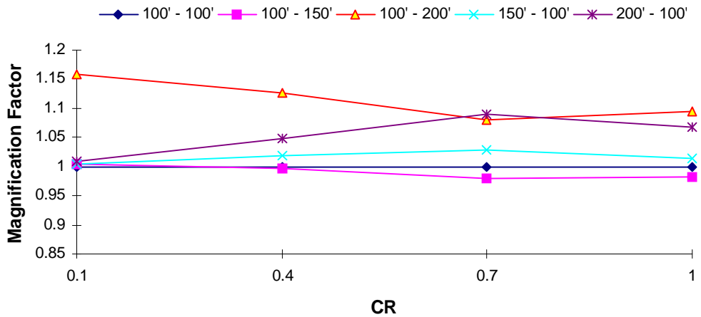
DOF 2 Magnification Factor : El Centro EQ T_1 = 3.0 s, TR = 1.0
