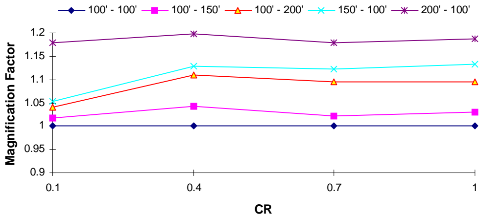
DOF 1 Magnification Factor : El Centro EQ T_1 = 3.0 s, T_R = 0.7
