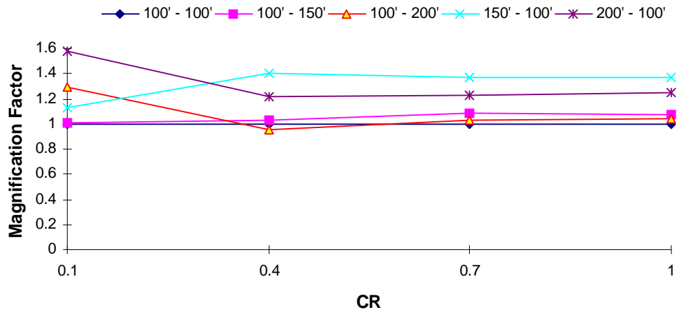
DOF 1 Magnification Factor : Northridge EQ T_1 = 3.0 s, T_R = 0.7
