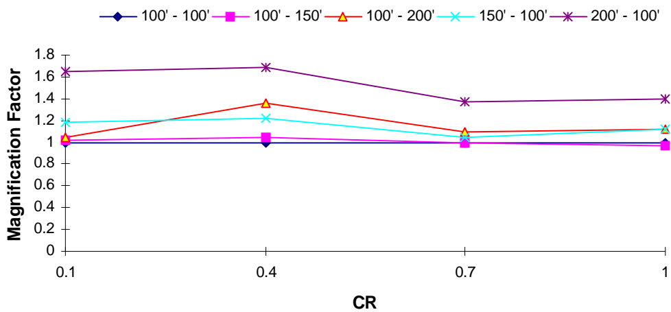
DOF 1 Magnification Factor : Northridge EQ T_1 = 3.0 s, TR = 1.0
