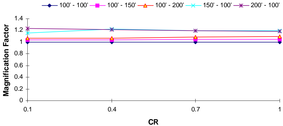
DOF 1 Magnification Factor : El Centro EQ T_1 = 3.0 s, TR = 0.4
